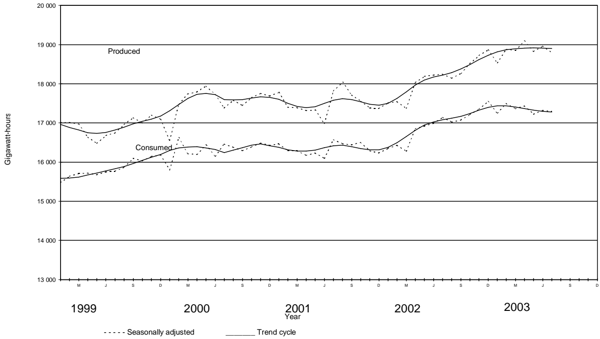
Figure 1 – Electricity consumed and produced in South Africa
