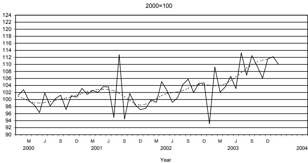
Figure 1 - Indices of physical volume of total mining production including gold
